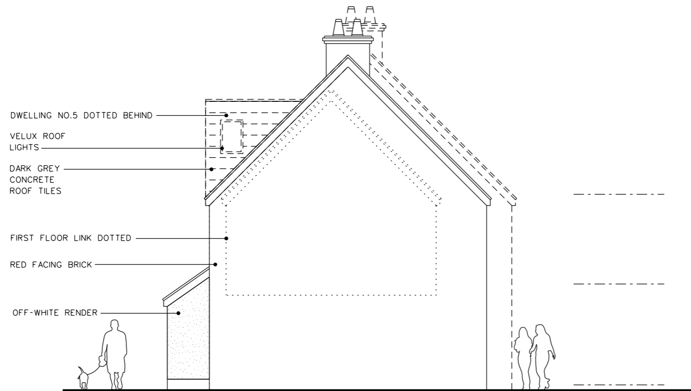
PROPOSED SIDE ELEVATION (DWELLINGS 1-4)
